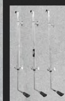
PMBDL3/C CHROME MULTI BASS DRUM LEGS Multi-Bass Drum Legs allow any bass drum to be played horizontally. Height and tilt adjustable. (Patent Pending)
