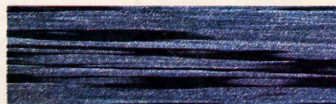
No. 17 GALAXY
